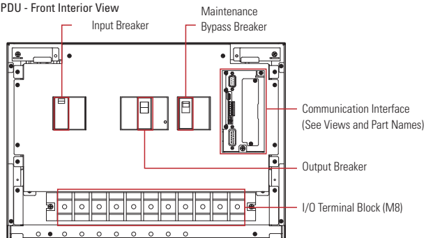
(3) PDU - Front Interior View
