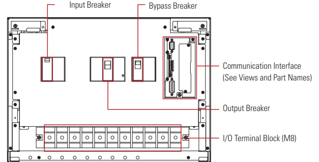
(3) PDU - Front Interior View
