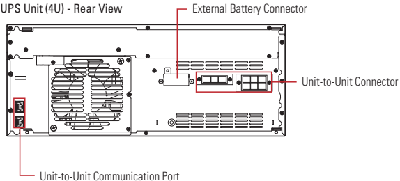
(2) UPS Unit (4U) - Rear View
