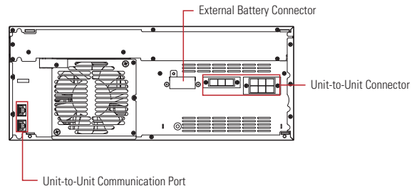
(1) UPS Unit - Rear View
